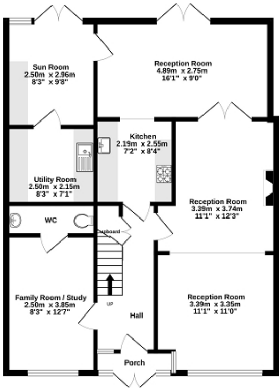
Ground Floor 73.7 sq.m. (794 sq.ft.) approx.
